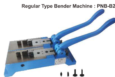
Regular Type Bender Machine : PNB-B2
